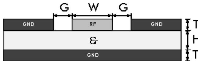
Figure7-8: Structure of a grounded CPWG
