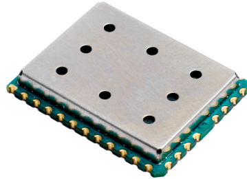
Figure 1-1: Picture of iMAS923TH; iM980A
