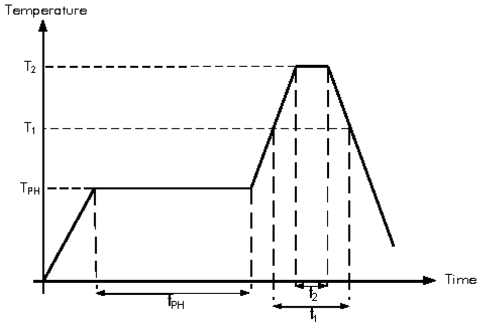
Figure7-9: Soldering Profile
