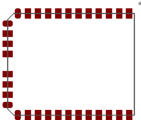
Figure5-6: Recommended footprint of the iMAS923TH; iM980A (top view)
