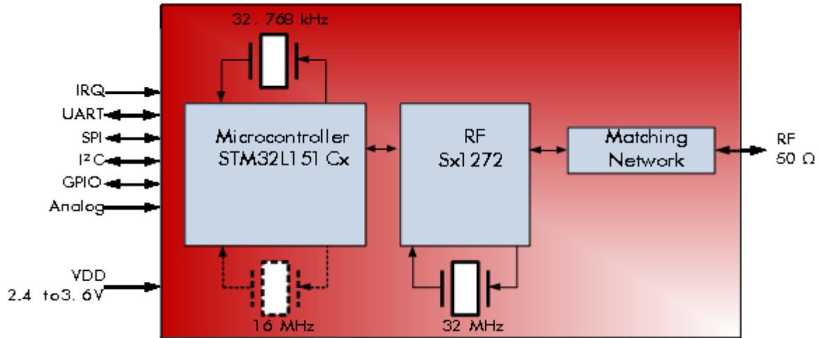
Figure 2-2: Block Diagram of Radio Module iMAS923TH; iM980A
