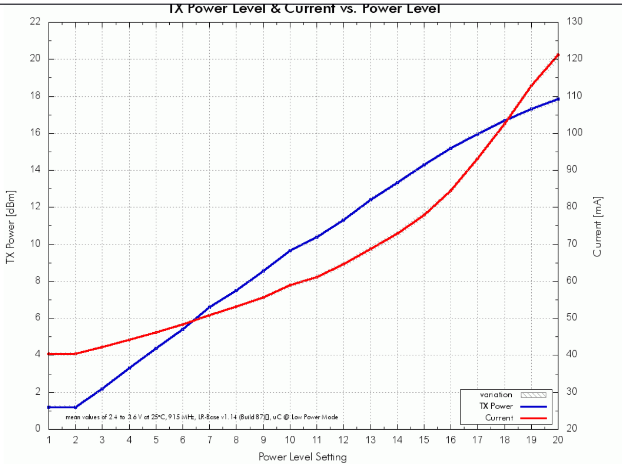
Figure4- 3: RF output power level and current consumption versus power stages from 1 to 20 @ room temperature
