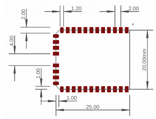
Figure5-5: Outer Dimensions of the iMAS923TH; iM980A (top view)
